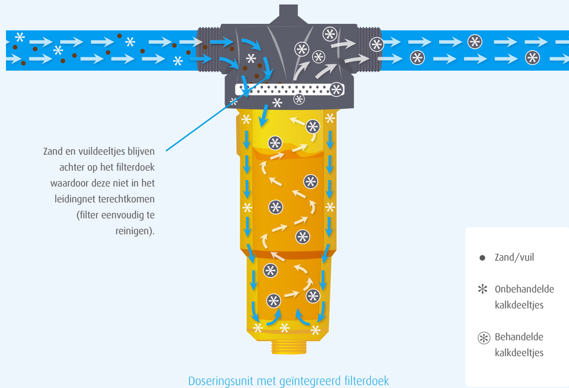
NoCalc CombiCompact NC38770
